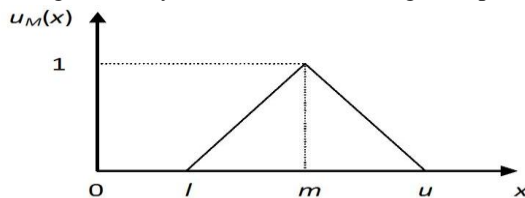
Figure 2 Triangular fuzzy numbers
